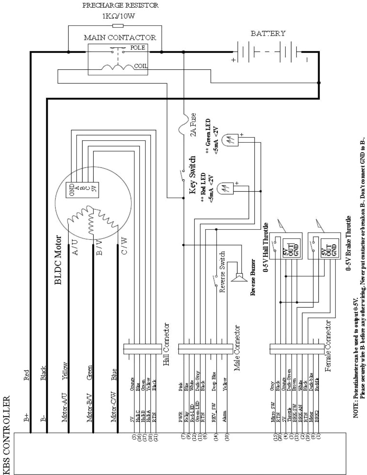
Figure 3: KBS controller standard wiring (Battery voltage can be used for controller supply)
