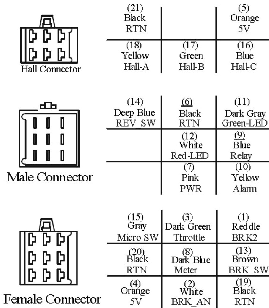
Figure 2: connector pin definition diagram
